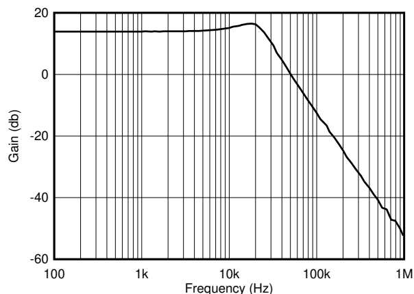
图 8-2. OPAx140 Second-Order, 25-kHz, Chebyshev, Low-Pass Filter
