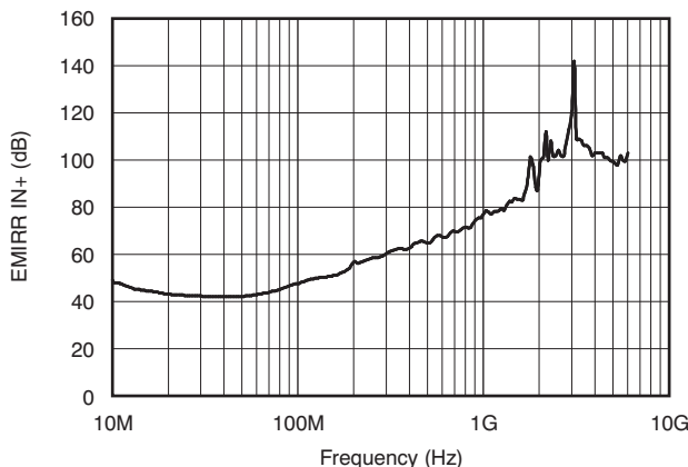
Figure 43. EMIRR Testing
