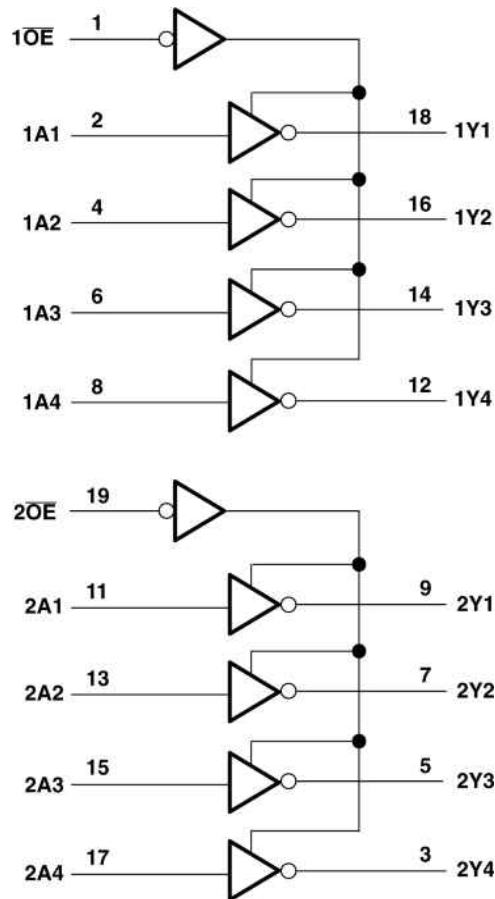
图 8-1. Logic Diagram (Positive Logic)
