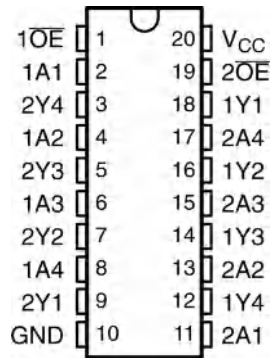
图 5-1. SN54AC240 J or W Package; SN74AC240 DB, DW, N, NS, or PW Package (Top View)
