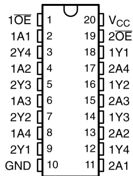
图 4-1. SN54AC244 J or W Package SN74AC244 DB, DW, N, NS, or PW Package (Top View)
