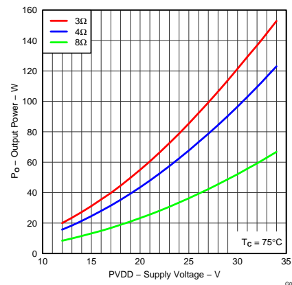
图 4. Output Power vs Supply Voltage, vs Distortion + Noise = 1%
