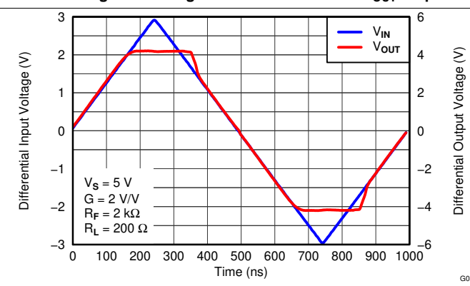
Figure 40. Overdrive Recovery
