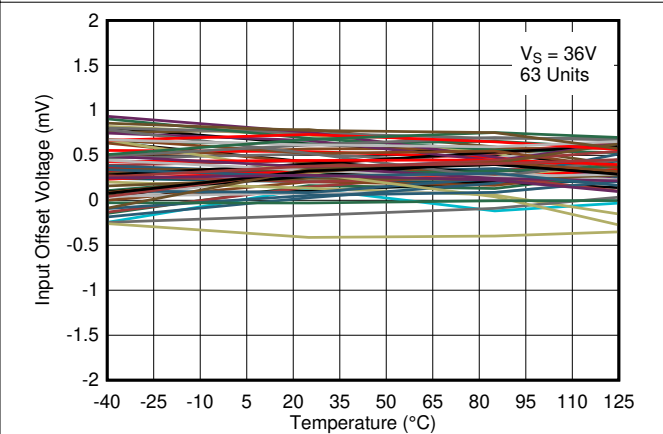
图 6-21. Input Offset Voltage vs. Temperature at 36V
