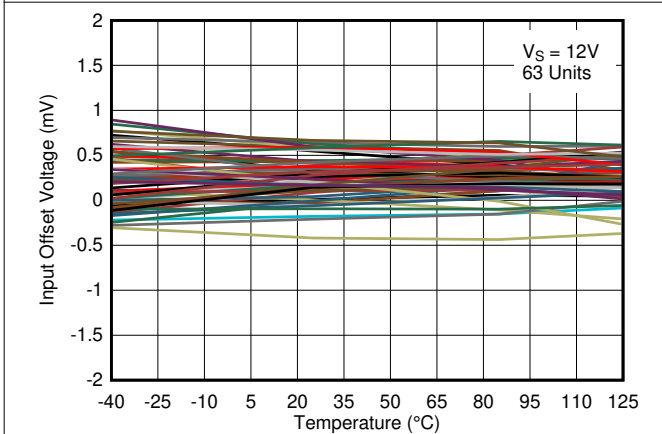
图 6-20. Input Offset Voltage vs. Temperature at 12V
