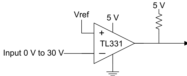
图 8-1. Typical Application Schematic
