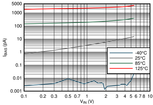
V_S = 1.8\text{V to }5\text{V} TLV40x1Ry 图 7-19. Bias Current vs Common Mode Voltage
