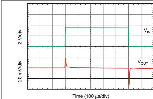
图 8-8. Line Transient Response
