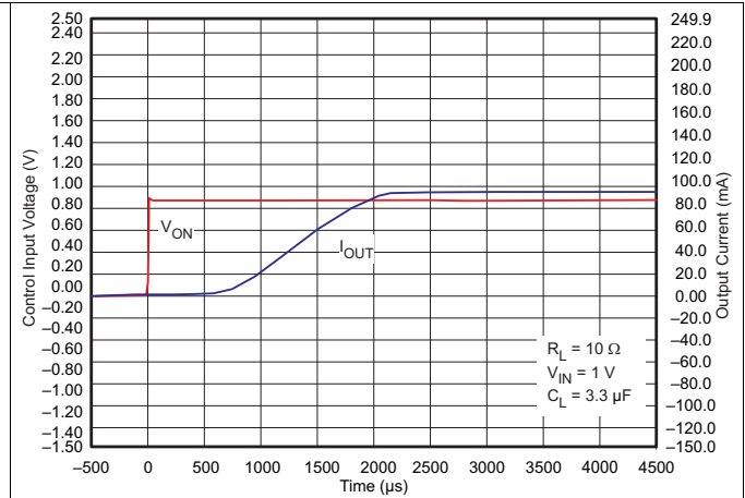
Figure 43. t_{ON} Response
