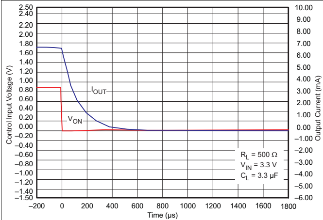
Figure 46. t_{OFF} Response
