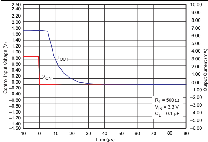
Figure 44. t_{OFF} Response
