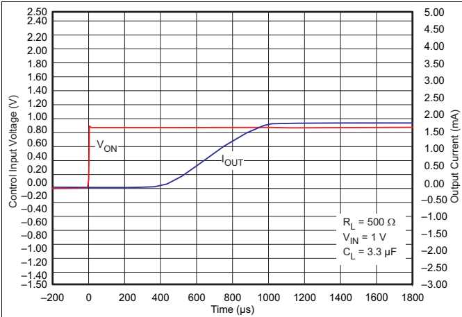
Figure 42. t_{ON} Response
