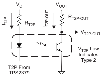
Figure 18. T2P Interface
