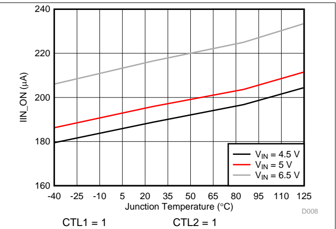
图 8. Enabled IN Supply Current – CDP (11) vs Temperature
