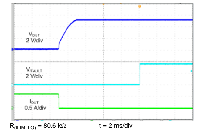
图 22. Short Circuit to No Load (SDP)
