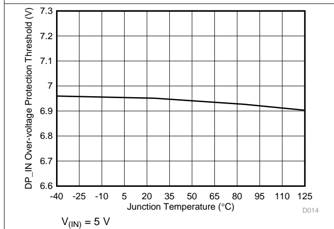
图 11. OUT Overvoltage Protection Threshold vs Temperature
