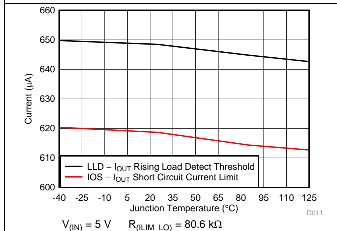
图 9. I_{(OUT)} Rising Load-Detect Threshold and OUT Short-Circuit Limit vs Temperature
