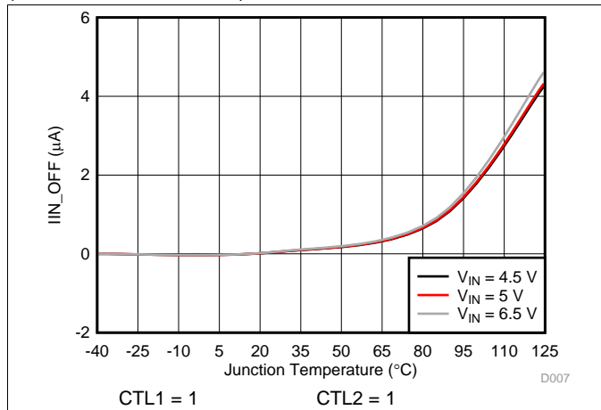
图 7. Disabled IN Supply Current vs Temperature
