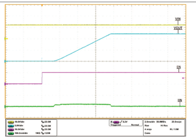
图 29. Output Voltage Ramp and Inrush Current at Start Up, C_{dvdt} = 22\text{ nF}
