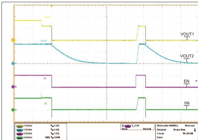
图 56. TPS259541 Self-controlled Mode Response with Overload Fault on OUT1 Followed by Auto-retry with Persistent Fault
