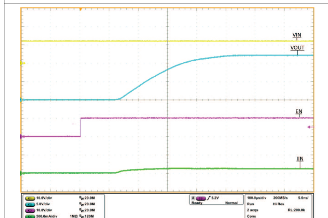
图 28. Output Voltage Ramp and Inrush Current at Start Up, C_{dvdt} = \text{Open}
