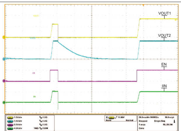
图 57. TPS259541 Self-controlled Mode Response with Overload on OUT1 Followed by Recovery with Fault Removed
