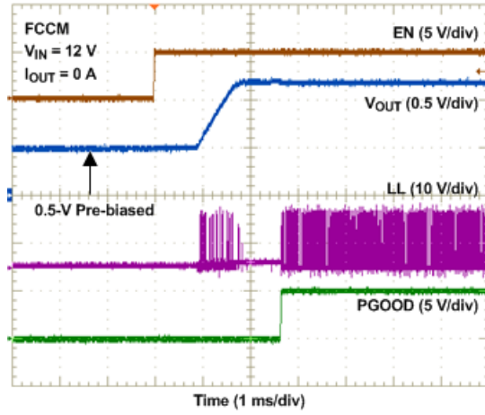
图 9-3. Pre-Bias Start-Up
