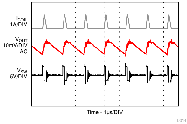
图 9-28. PSM Operation
