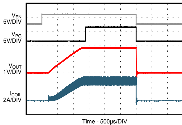
图 9-30. Start-Up with No-Load
