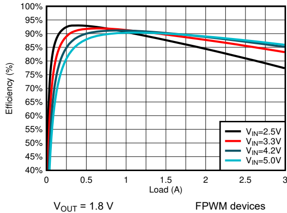
图 9-17. Efficiency
