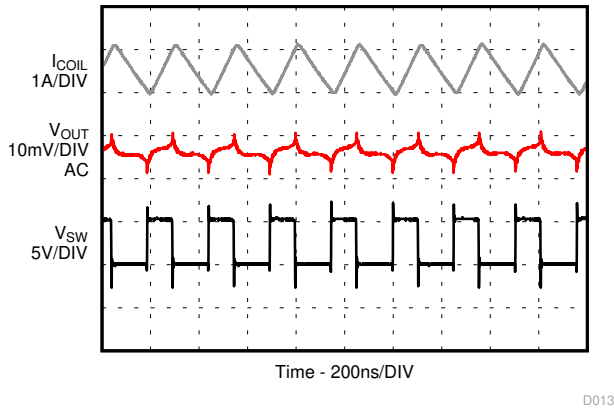
图 9-27. PWM Operation
