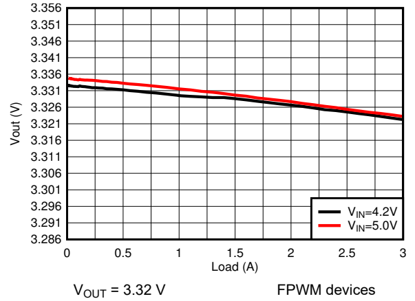
图 9-22. Load Regulation
