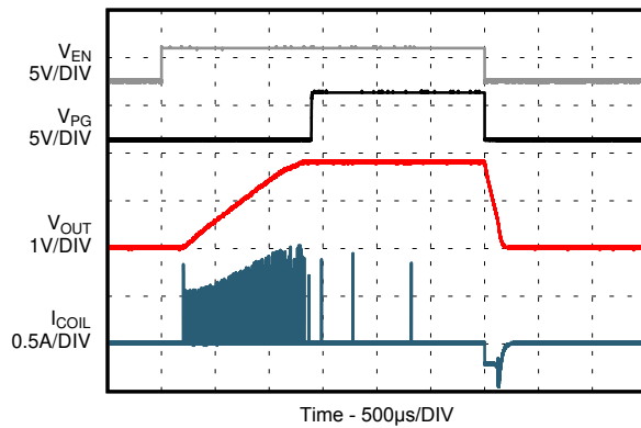
图 9-28. PSM Operation
