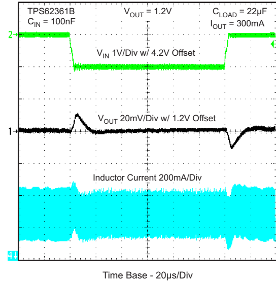
LINE TRANSIENT RESPONSE V_{IN} RANGE: 4.2V to 3.2V
