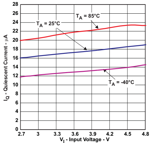
Figure 14. Quiescent Current vs Input Voltage
