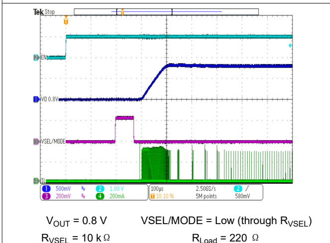
图 9-38. TPS62801 Start-Up, V_{OUT} = 0.8\text{ V}
