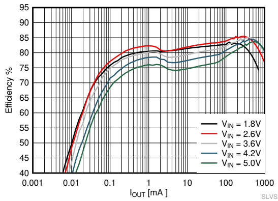
TPS62801 R_{VSEL} = 10\text{ k}\Omega to GND 图 9-4. Efficiency Power Save Mode V_{OUT} = 0.8\text{ V}
