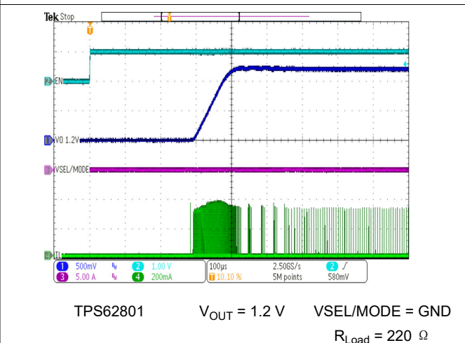
图 9-39. Start-Up, V_{OUT} = 1.2\text{ V}
