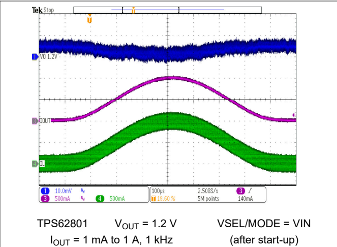
图 9-35. AC Load Sweep Forced PWM Mode
