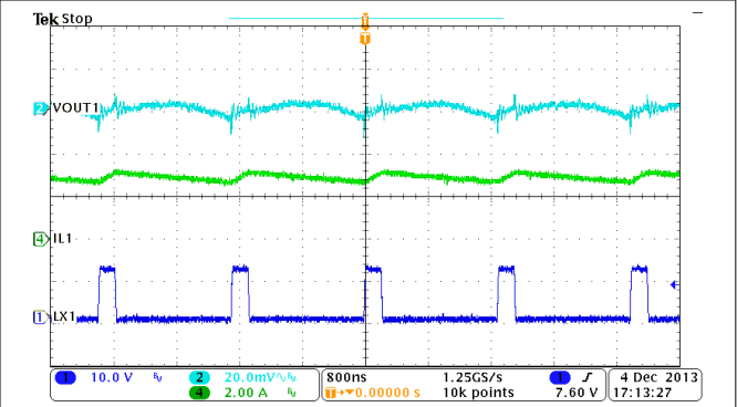
图 9-9. Buck1, Steady State Operation at Full Load
