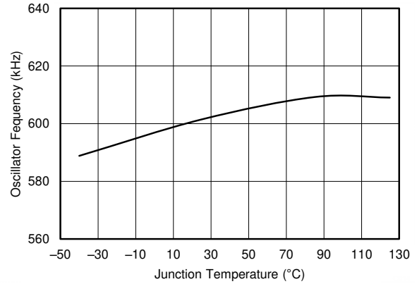
图 7-14. Oscillator Frequency vs Temperature
