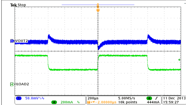
图 9-16. Buck2, Load Transient, 0.25 to 0.5 A SR = 0.25 A/µs
