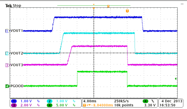
图 9-27. Automatic Power Sequencing, MODE = EN1 = EN2 = HIGH
