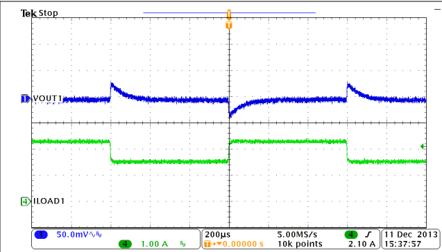
图 9-15. Buck1, Load Transient, 1.5 to 2.25 A SR = 0.25 A/µs
