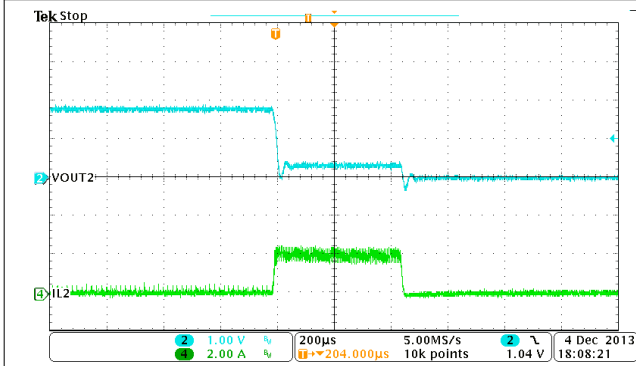
图 9-22. Buck2, OCP
