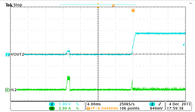
图 9-23. Buck2, Hiccup and Recovery
