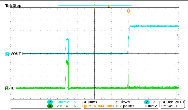
图 9-21. Buck1, Hiccup and Recovery
