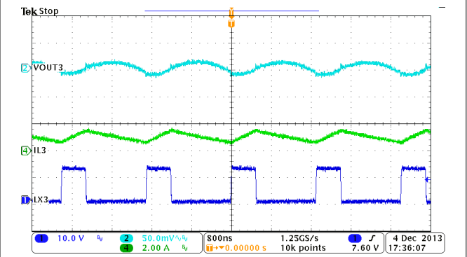
图 9-13. Buck3, Steady State Operation at Full Load
