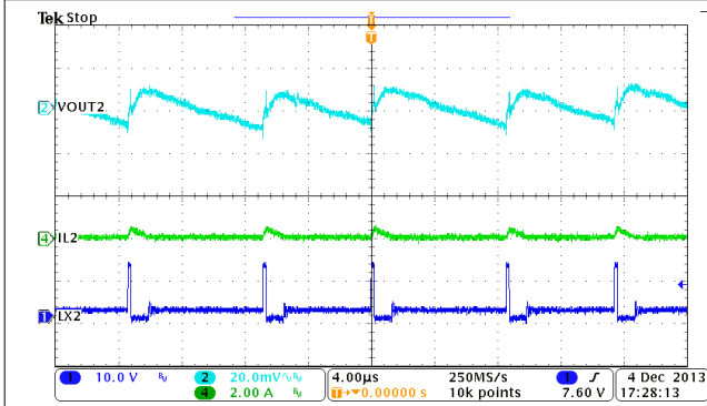
图 9-10. Buck2, Steady State Operation at Light Load
