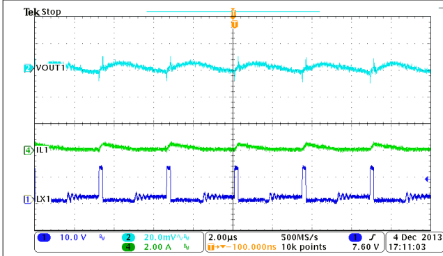
图 9-8. Buck1, Steady State Operation at Light Load
