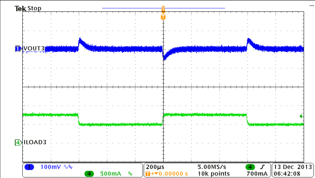
图 9-19. Buck3, Load Transient, 0.5 to 0.75 A SR = 0.25 A/µs
