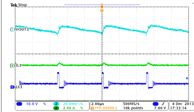
图 9-12. Buck3, Steady State Operation at Light Load
