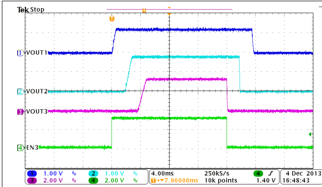
图 9-26. Automatic Power Sequencing, MODE = EN1 = EN2 = HIGH
