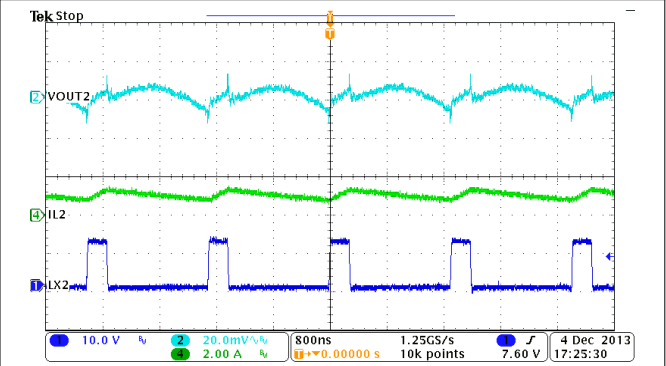
图 9-11. Buck2, Steady State Operation at Full Load
