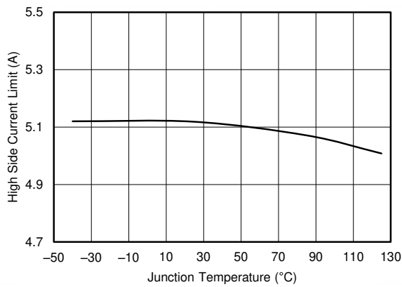
图 7-21. Buck1 High-Side Current Limit vs Temperature
