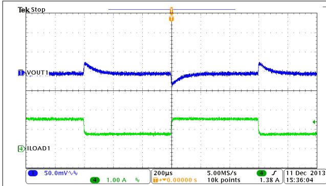
图 9-14. Buck1, Load Transient, 0.75 to 1.5 A SR = 0.25 A/µs
