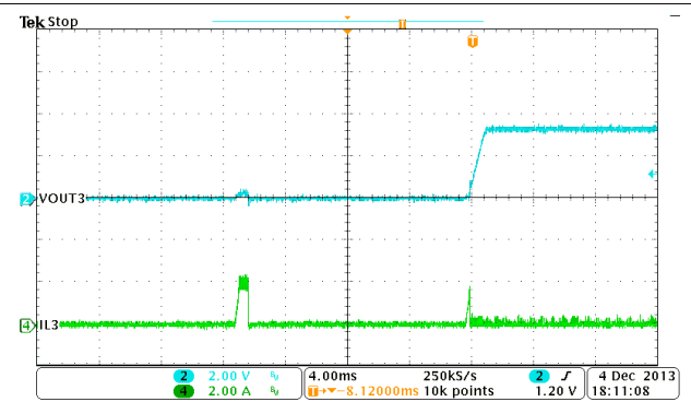
图 9-25. Buck3, Hiccup and Recovery
