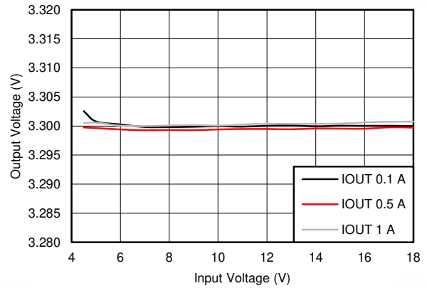
图 7-8. BUCK3, Line Regulation
