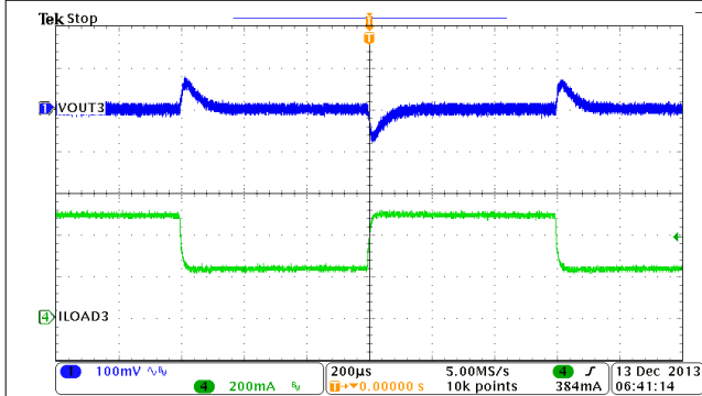
图 9-18. Buck3, Load Transient, 0.25 to 0.5 A SR = 0.25 A/µs
