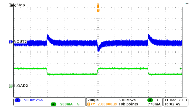
图 9-17. Buck2, Load Transient, 0.5 to 0.75 A SR = 0.25 A/µs
