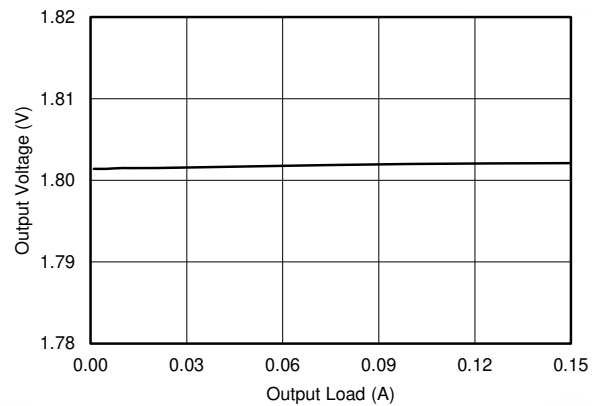
图 7-10. LDO2, Load Regulation
