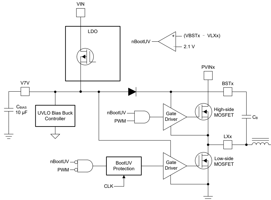
图 8-5. V7V Linear Dropout Regulator and Bootstrap Voltage Diagram
