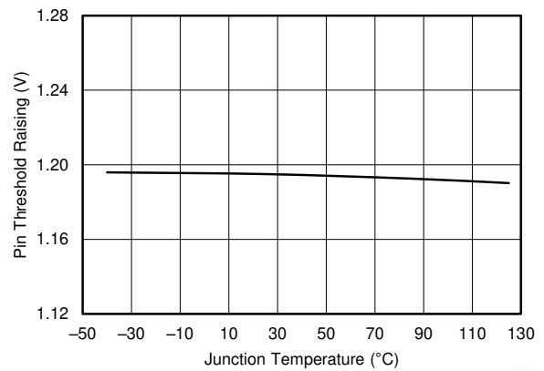
图 7-18. EN Pin Threshold Rising vs Temperature
