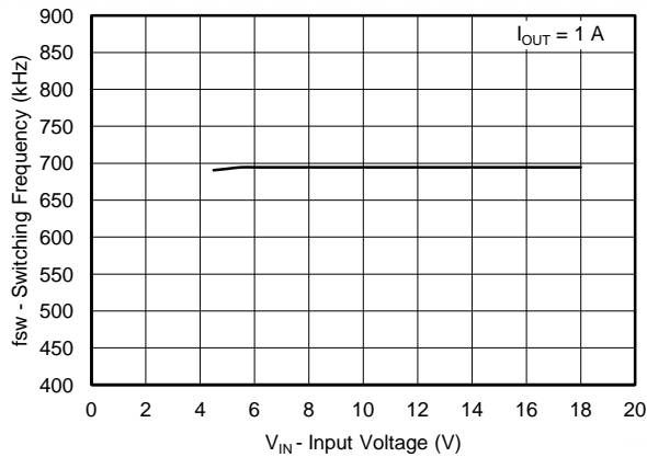
Figure 22. V OUT3 = 1.5V Switching Frequency vs Input Voltage
