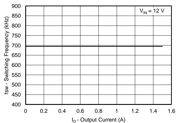
Figure 25. V OUT3 = 1.5V, Switching Frequency vs Output Current
