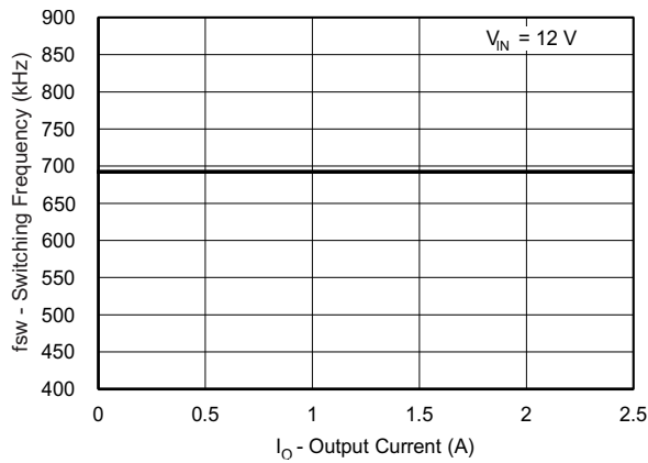
Figure 24. V OUT2 = 1.2V, Switching Frequency vs Output Current
