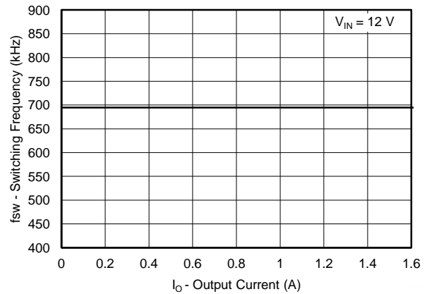
Figure 23. V OUT1 = 3.3V Switching Frequency vs Output current
