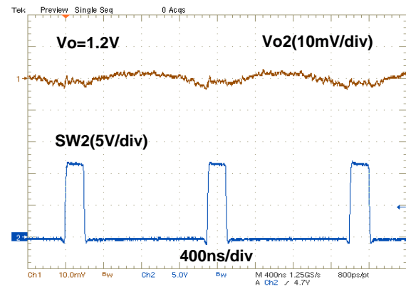
Figure 27. V OUT2 = 1.2V, Ripple Voltage at I OUT2 = 2.5A
