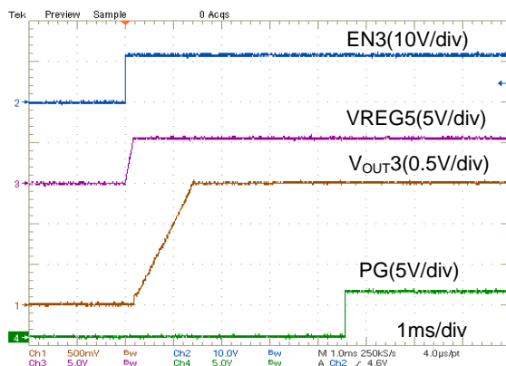
Figure 34. VOUT3 = 1.5V Soft-Start IOU3 = 1.5A
