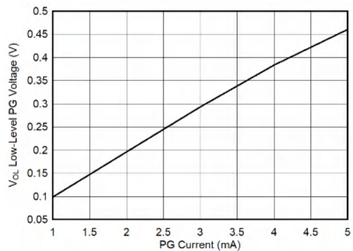
图 6-40. Low-Level PG Voltage vs Current
