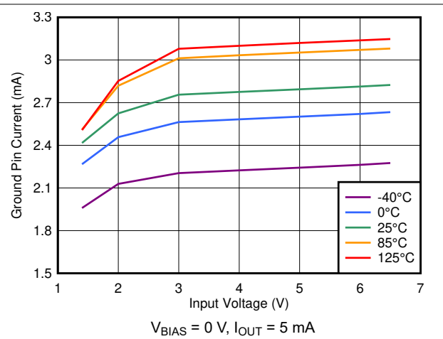
图 7-32. Ground Pin Current vs Input Voltage
