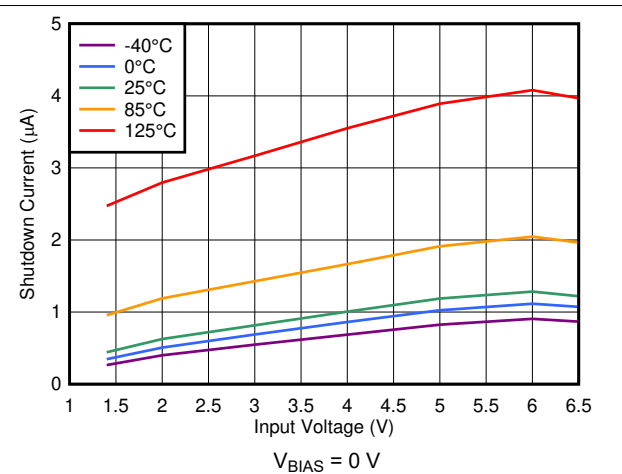
图 7-34. Shutdown Current vs Input Voltage
