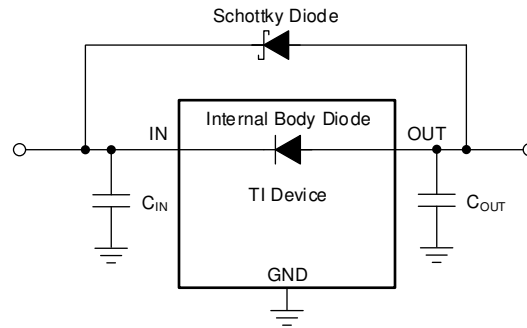
图 9-13. Example Circuit for Reverse Current Protection Using a Schottky Diode
