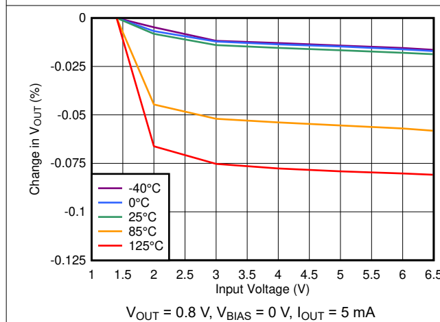
图 6-29. Line Regulation Without Bias
