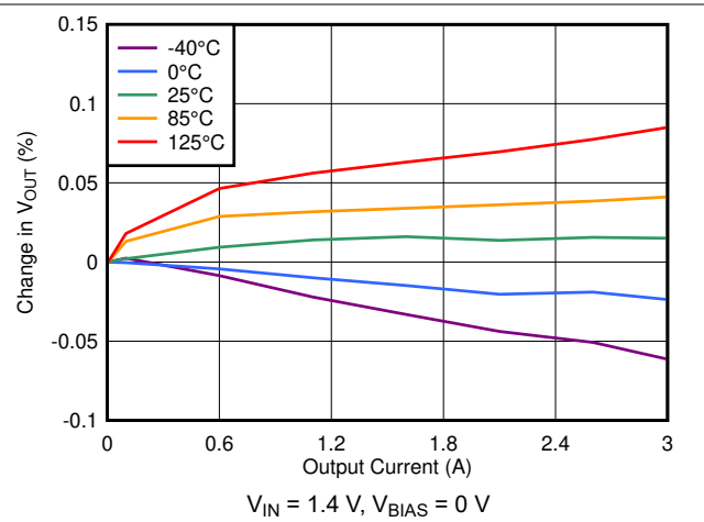
图 6-26. Load Regulation With Bias
