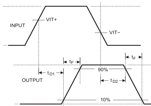
Figure 2. Timing Diagram
