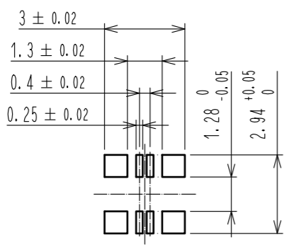
RECOMMENDED PCB LAYOUT (5:1)
