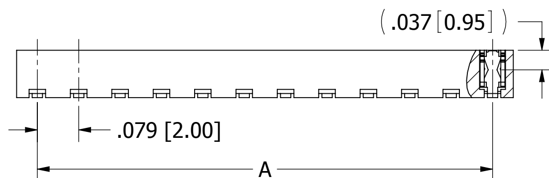
SFM230-NPPN-S__-SD-BK (OPPOSITE BEND, APPLICABLE ON EVEN PIN COUNTS)
