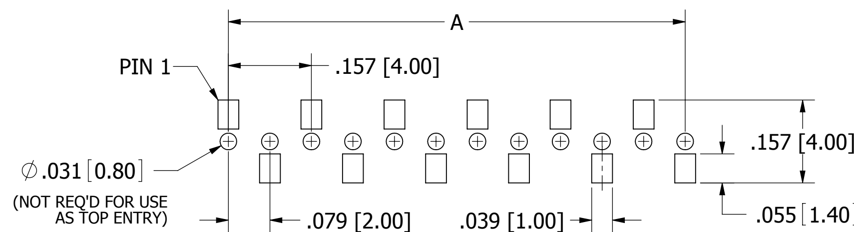
RECOMMENDED PCB LAYOUT SFM230-NPPN-S__-SC-BK
