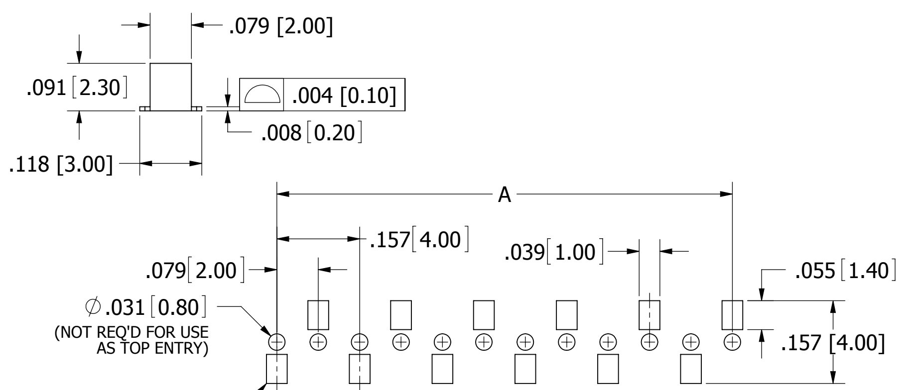
RECOMMENDED PCB LAYOUT SFM230-NPPN-S__-SD-BK
