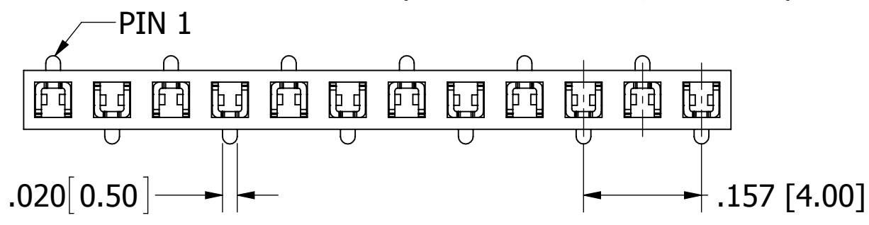
SFM230-NPPN-S__-SC-BK (STANDARD)
