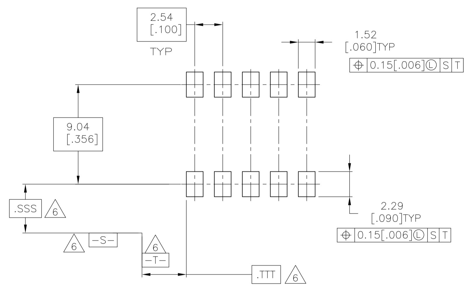
RECOMMENDED PC BOARD LAYOUT
